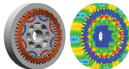
Traction motor
